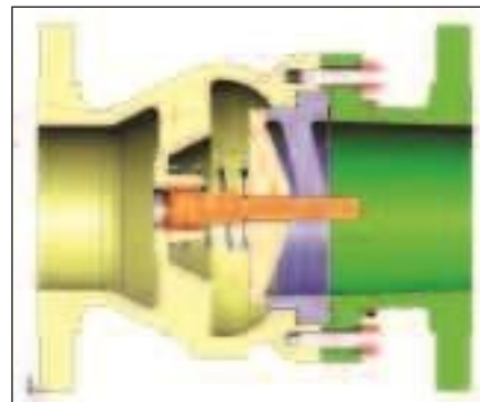
Shown here is an example of an in-line check valve. This valve is also known as a nozzle check or silent check valve.
